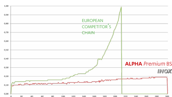
Wear test comparing an Alpha Premium STAINLESS STEEL chain with a top range European stainless steel chain
