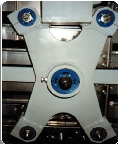
Heat resistant double rockers for pasta dryers
