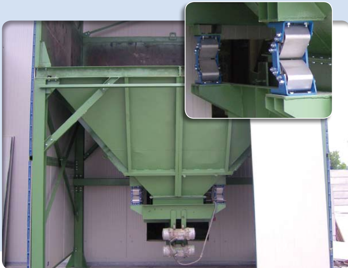
Hanging installation of feeders on bunker silos
