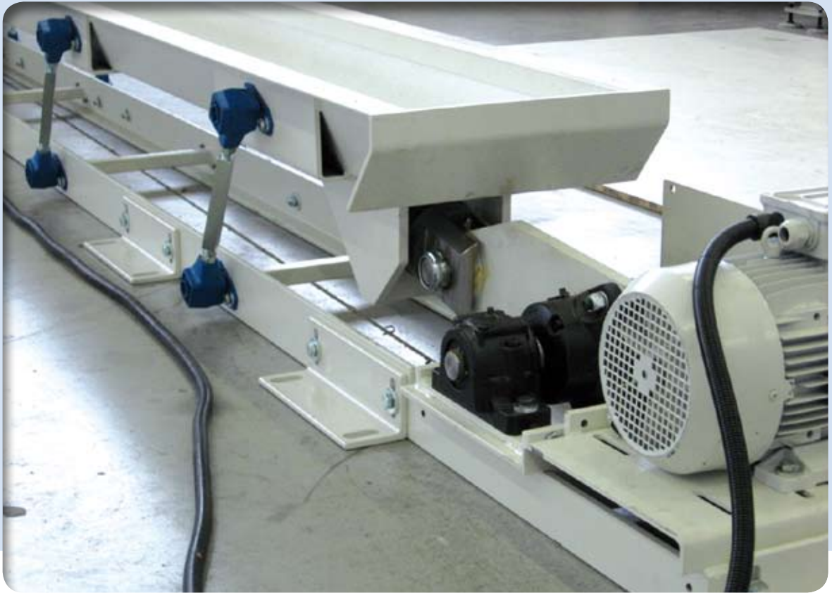
Rocker suspensions for conveyor troughs
