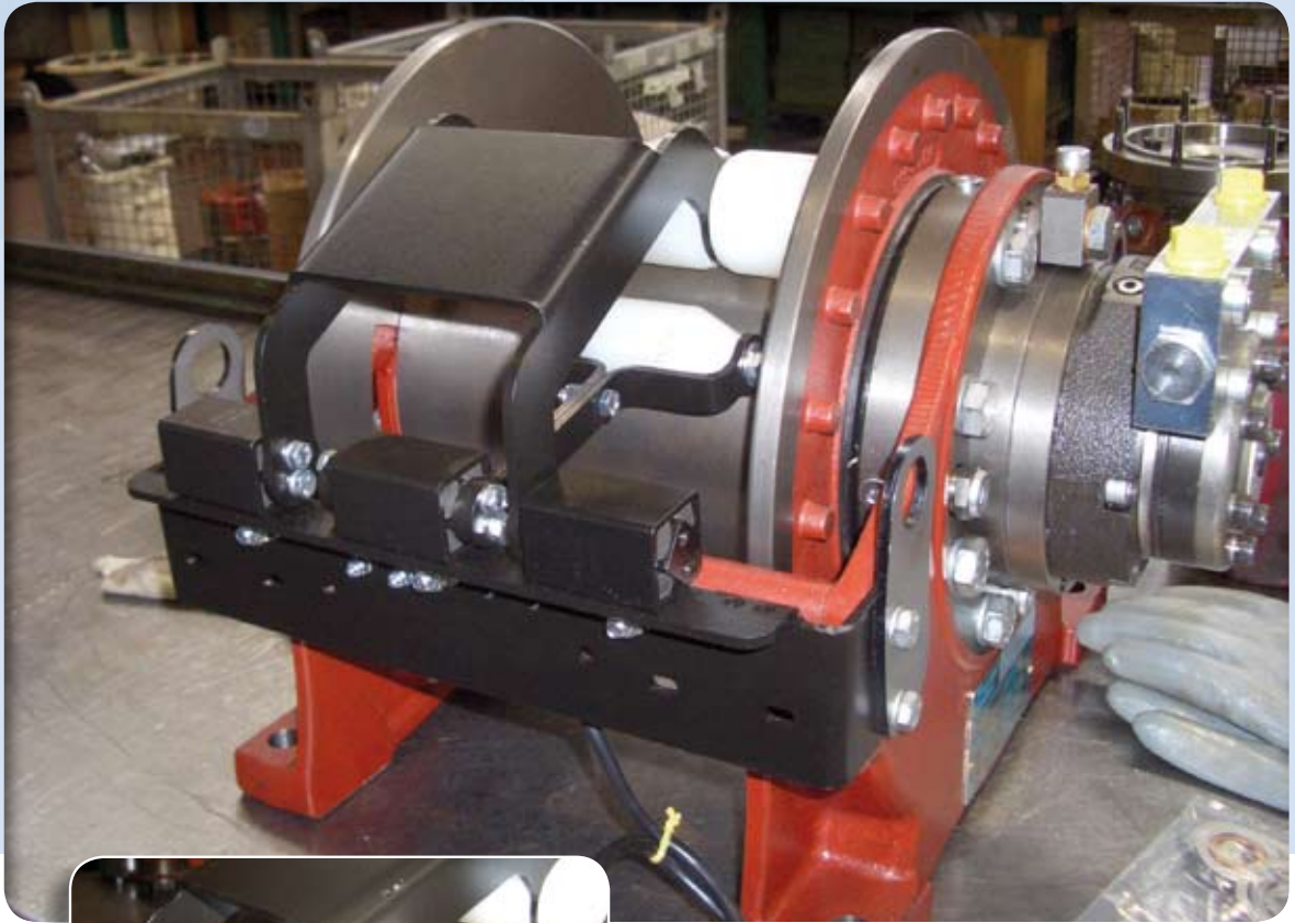
Guide roller suspensions for controlled cable reeling on winch drum
