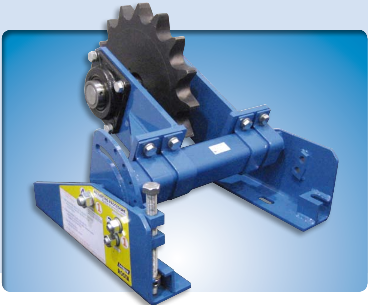
▲ Heavy Duty chain tensioner
