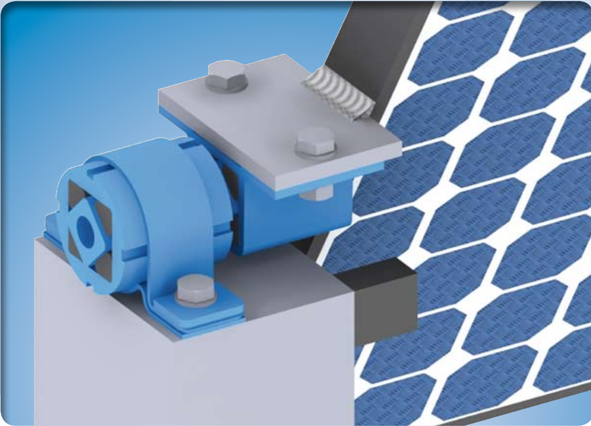
Elastic swivel mount for solar panels to compensate hard wind gusts
